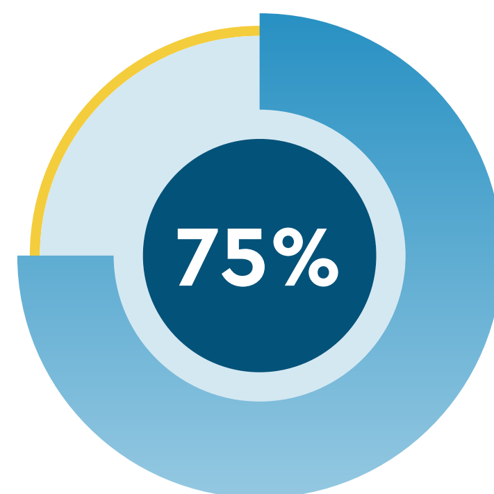
FOSSIL FUELS DRIVE CLIMATE CHANGE
